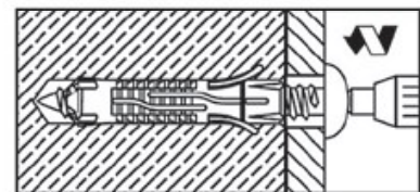
Drive screw into anchor.
