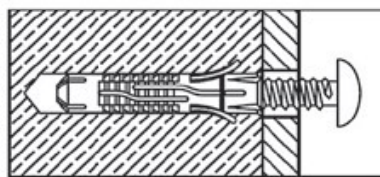
Install anchor.
